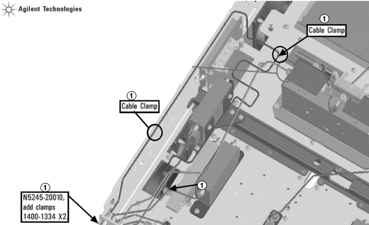
Figure 4 Location of Cable Clamps to Secure W33 (N5245-20010)
